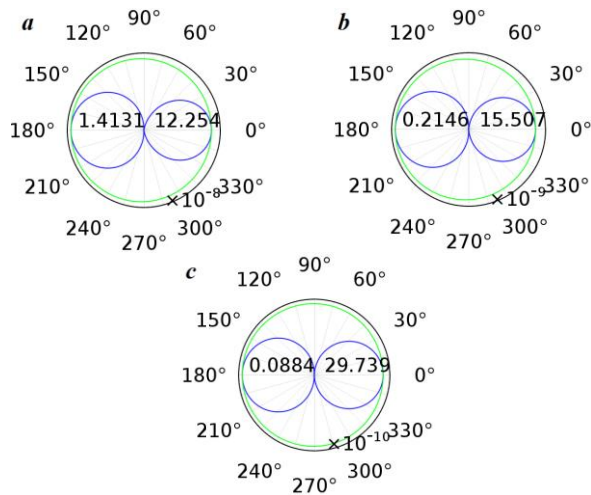
Fig. 2; (a) The far-field radiation pattern in the E-plane (blue) and H-plane (green) when wavelength is 400 nm, for Radius 10 nm (b) 50 nm (c) 100 nm, gold sphere. Due to symmetry, only one-quarter of the sphere has to be modeled (3D).
