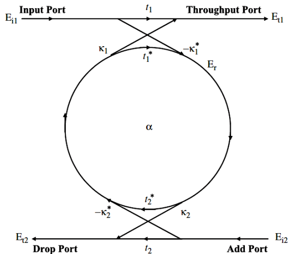
Figure 3: Model of a basic add/drop single MRR filter.
