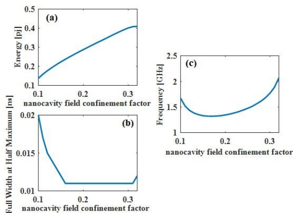
Fig. 4: (a) the energy, (b) FWHM; and (c) the frequency of the output signal versus \Gamma_c variations
