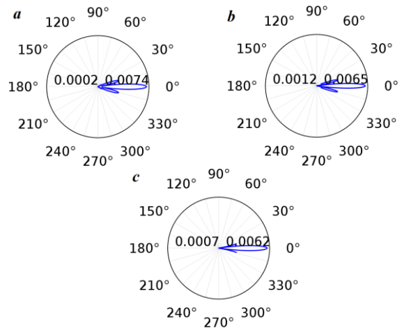
Fig. 4; Far-field norm & The far-field radiation pattern for (a) 1 Nano particle (b) 4 nanoparticles (c)10 nanoparticles, wavelength is 400 nm, Radius 50nm distance between particles 0.35\lambda , gold spheres (2D).
