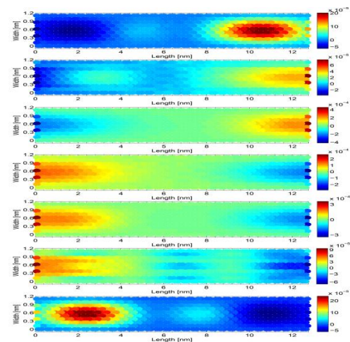
Fig. 4: Local photocurrent across the photodetector with Au-Ti leads under biasing conditions of V_{DS}=0 and V_{GS}= (a) -80 mV, (b) -40 mV, (c) -20 mV, (d) 0, (e) 20 mV, (f) 40 mV and (g) 80 mV. Color bars indicate the local currents in units of \mu\text{A} .
