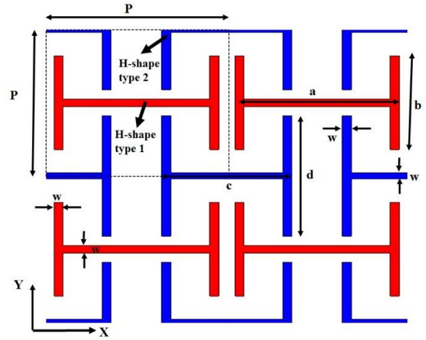
Figure 1: Schematic illustration of the plasmonic metamaterial.
