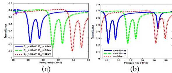
Fig. 4. The spectral response of the graphene sheets with different (a) Fermi energy for h=100\text{ nm} and (b) grating period for \Lambda=150\text{ nm} , h=100\text{ nm} , W=75\text{ nm} , E_{F1}=0.49\text{eV} , and E_{F2}=0.48\text{eV} .
