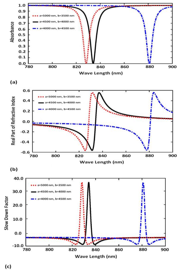
Figure 2: Numerical simulation of the ellipse shape proposed 2x2 plasmonic Metal/Dielectric/Metal (MDM)-structure wave guide ring oscillator-based slow light to show through the wave plasmonic cross from the waveguide coupling with oscillating wave. Dimension of this design is the micrometer scale.
