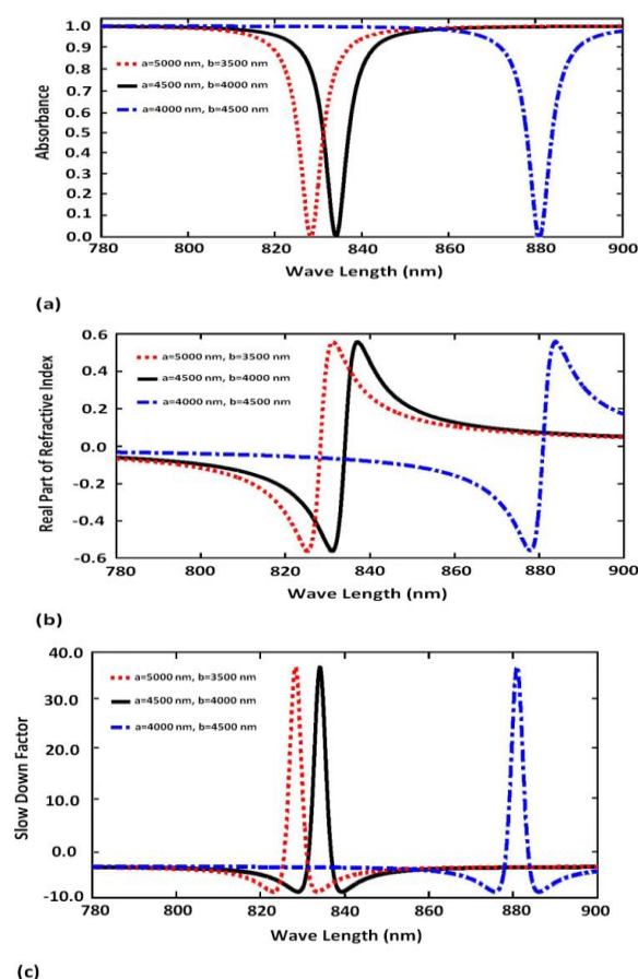
Figure 2: Numerical simulation of the ellipse shape proposed 2x2 plasmonic Metal/Dielectric/Metal (MDM)-structure wave guide ring oscillator-based slow light to show through the wave plasmonic cross from the waveguide coupling with oscillating wave. Dimension of this design is the micrometer scale.
