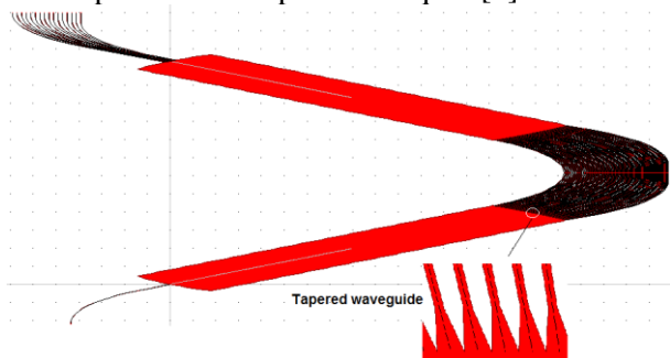
Figure 1: Schematic diagram of AWG. Waveguides connections to star couplers are tapered.
