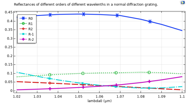
Fig. 2: Spreading of incident power over the diffraction orders in the plane grating.
